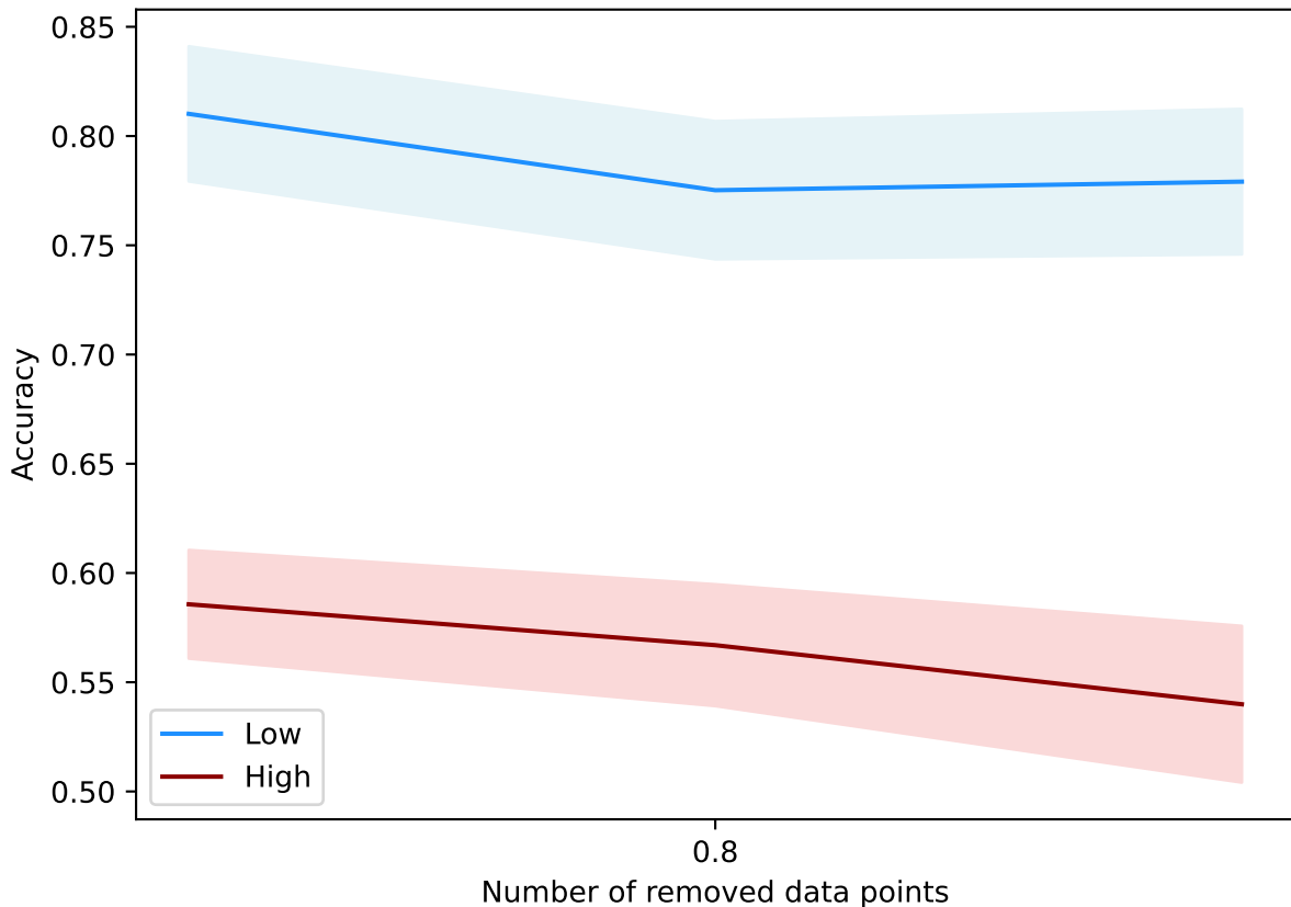
DataAttrOpt(10000, 0.2, 15, best, +b, alpha=best) - pol
